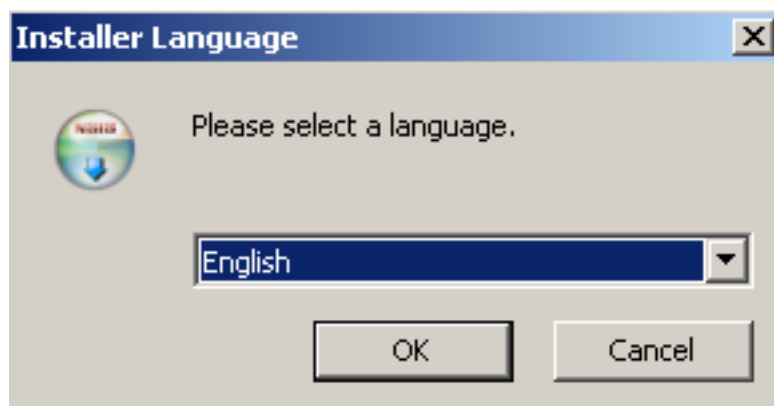
Figure 1: Language selection
